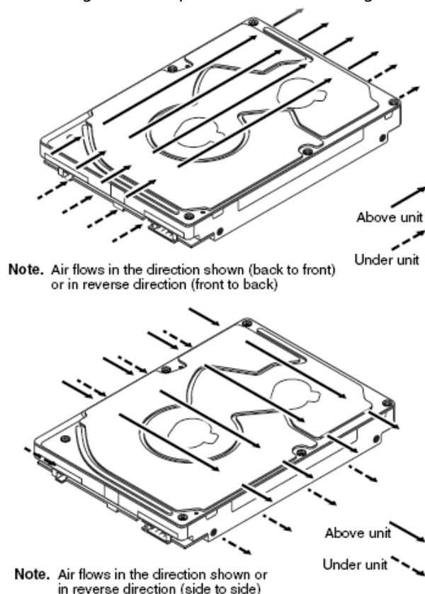
Figure 13. Air flow
