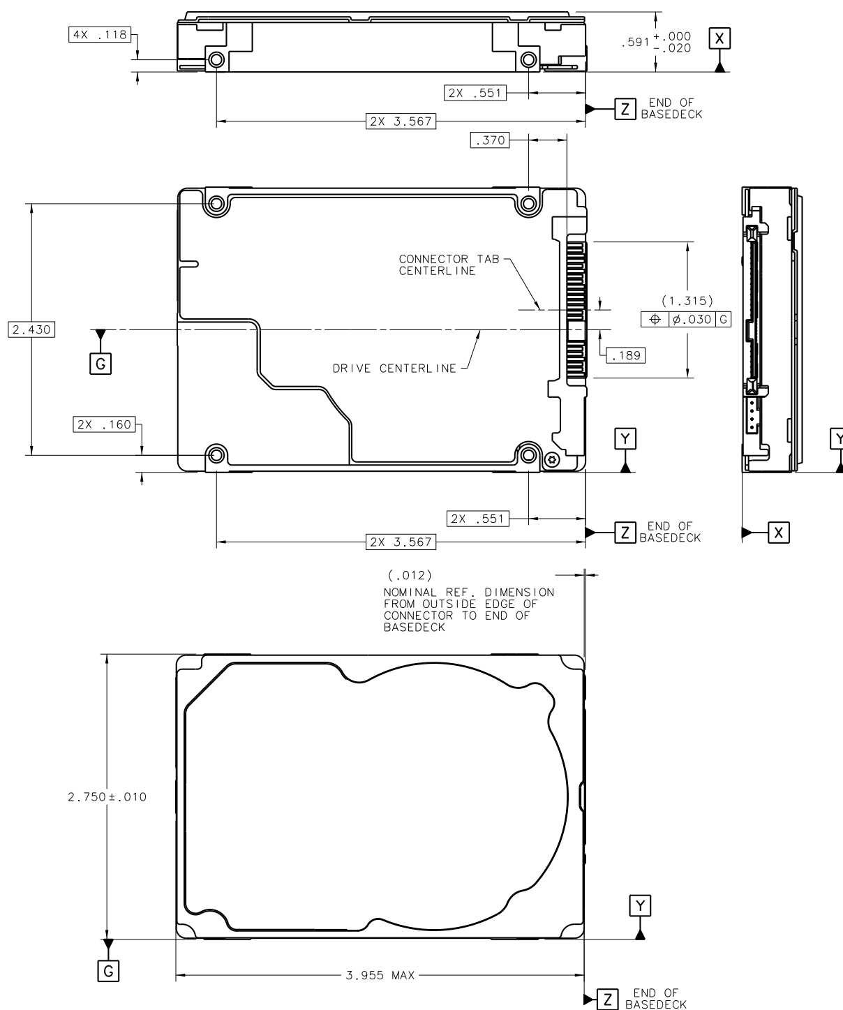
Figure 10. Mounting configuration dimensions
