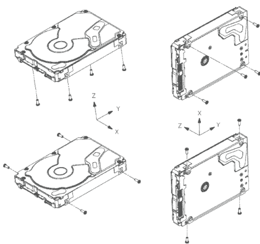
Figure 9. Recommended mounting
